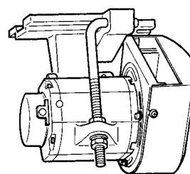
M91 small-sized motor unit (separately-available article)
